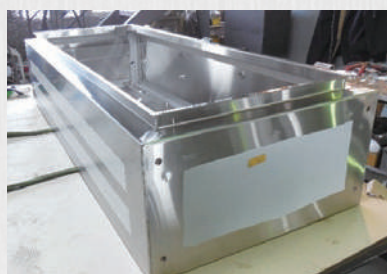
BOX w1200xL300xH600 t2(SUS304 HL)
